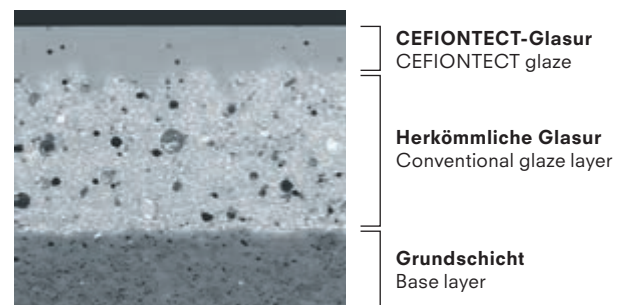
CEFIONTECT WC-Mikrograph * 1\ \mu\text{m} = 0,001\ \text{mm} CEFIONTECT toilet micrograph * 1\ \mu\text{m} = 0,001\ \text{mm}
